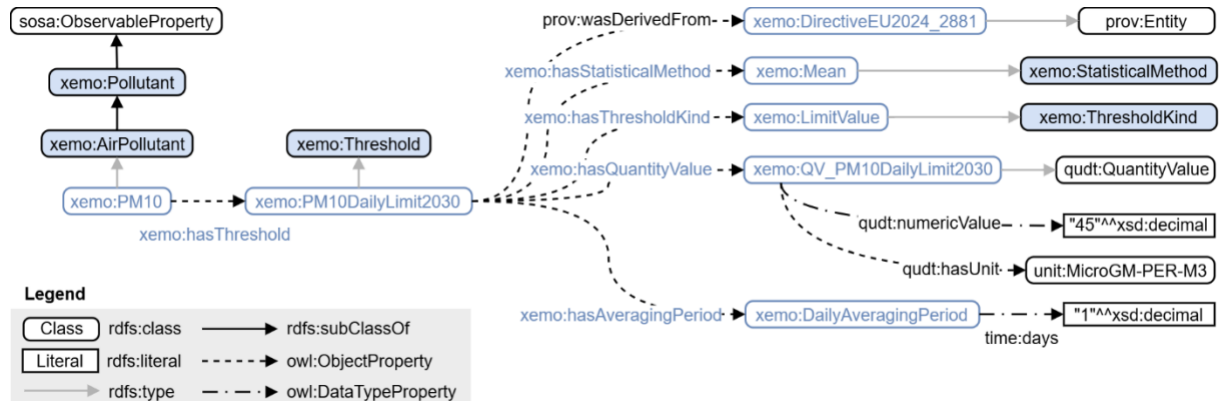
Figure 3: Graph representation of the PM 10 daily mean threshold applicable from 1 January 2030 under Directive (EU) 2024/2881, modelled in XEMO (original classes, properties, and individuals are shown in blue).
