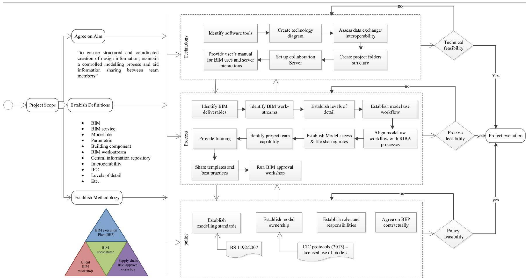
FIG. 6: Flat top-level view of the BIM protocols.
